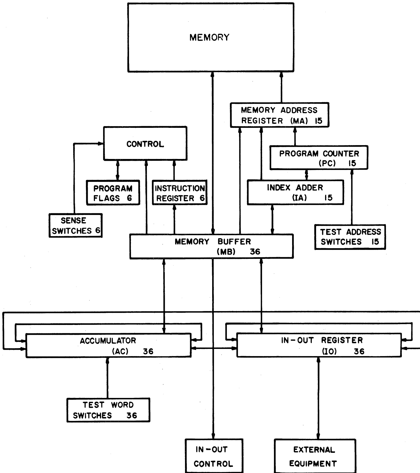
SYSTEM BLOCK DIAGRAM
